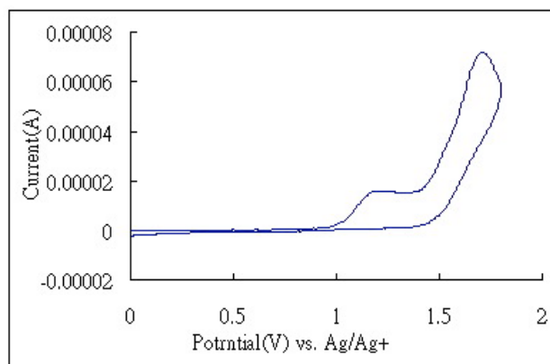
Figure 3. Cyclic voltammogram of 5e in CH 2 Cl 2 containing 0.1 M TBAPF 6 at a scan rate of 0.01 eV/s.
