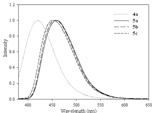
Figure 1. Normalized Photoluminescence Spectra of 4a , 5a , 5b , and 5c in CHCl 3 solution.
