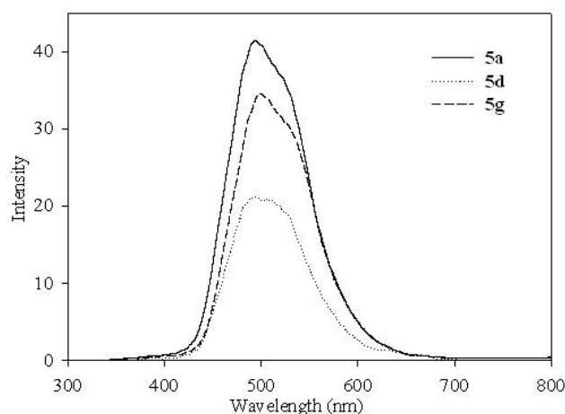
Figure 2. Normalized Photoluminescence Spectra of 5a , 5d , and 5g (Vacuum evaporated Film).
